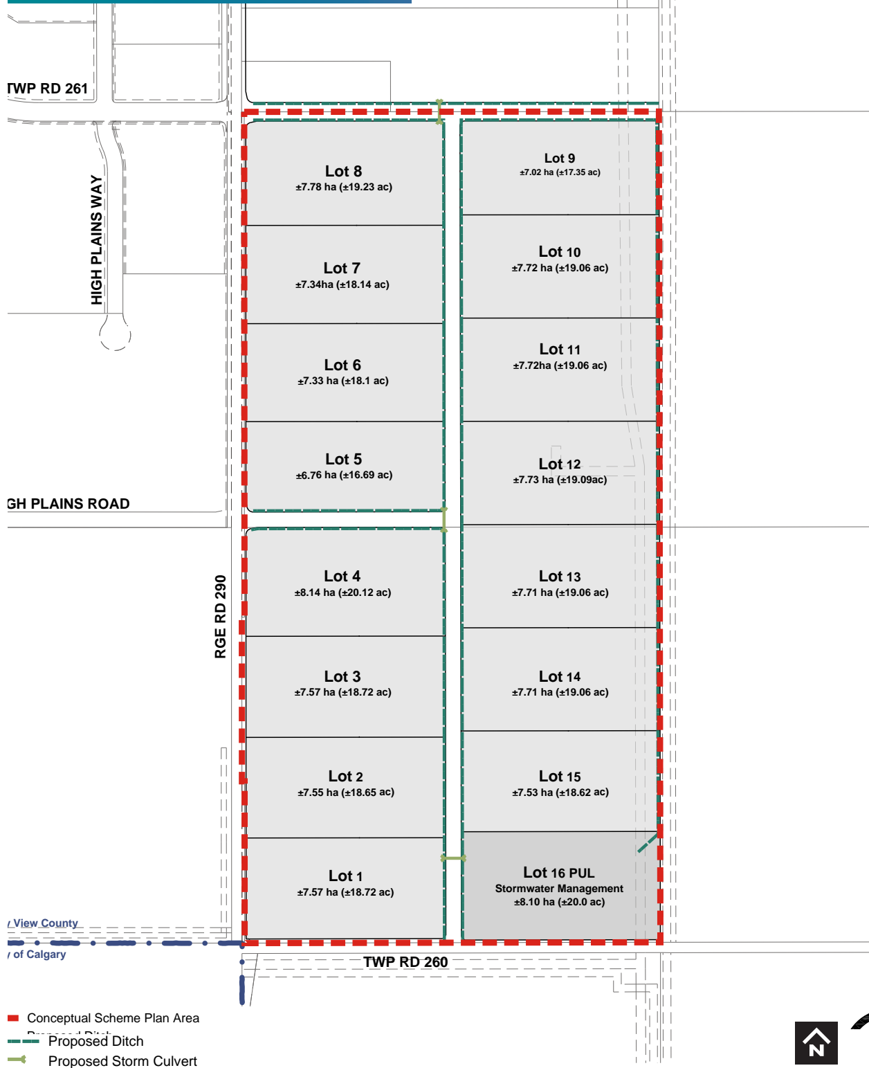
FIGURE 12: STORMWATER MANAGEMENT
