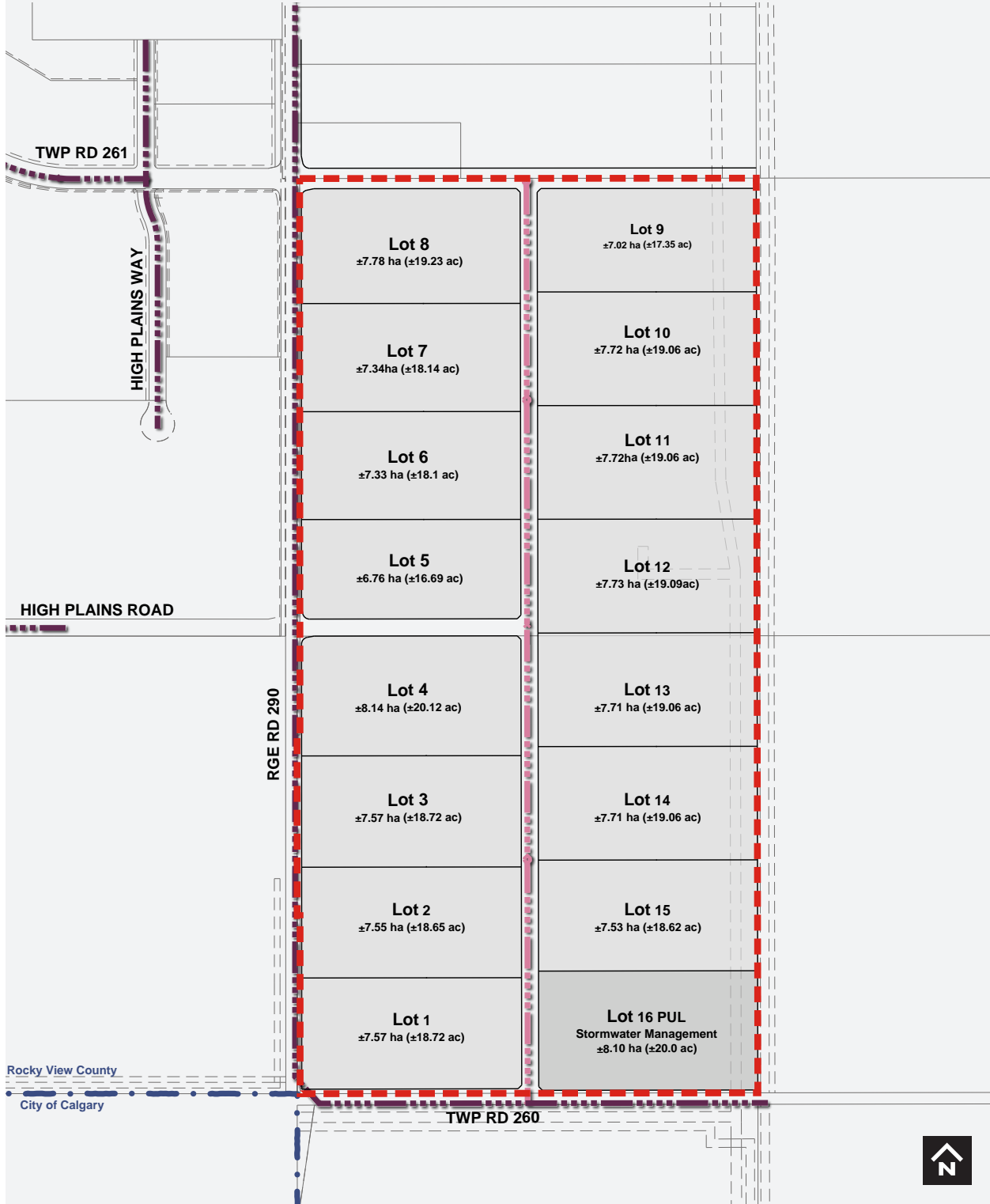
FIGURE 11: WASTEWATER SERVICING
