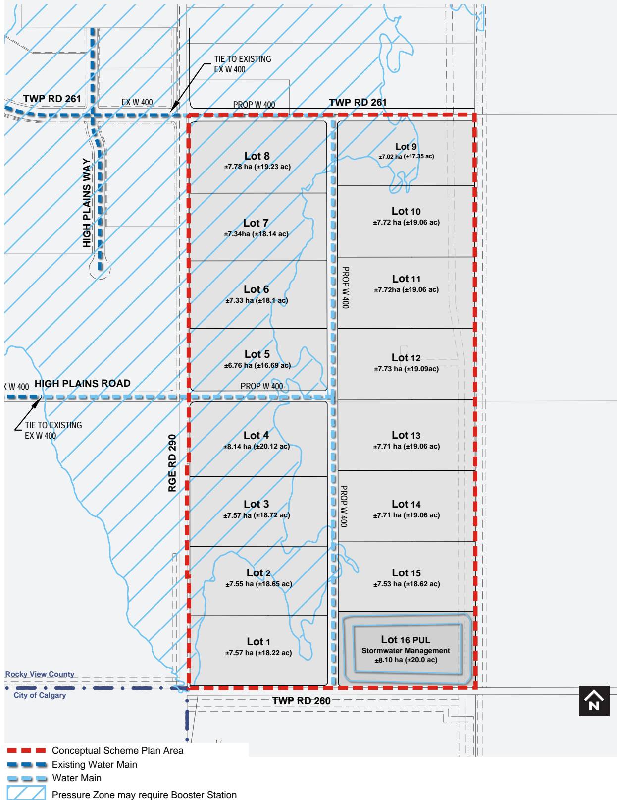
FIGURE 10: POTABLE WATER
