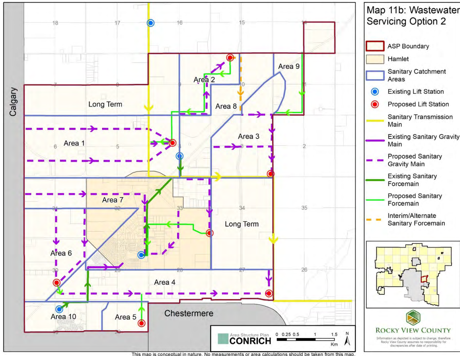
MAP 11B: Wastewater Servicing Option 2
