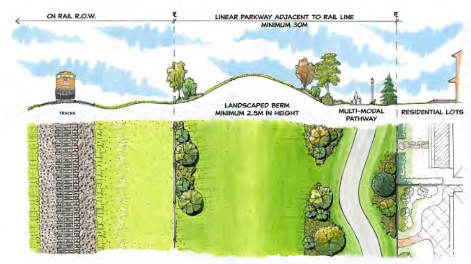
Figure 3 Railway interface concept
