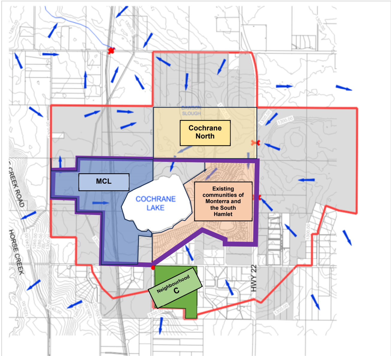
Map - Cochrane Lake Sub-Catchment Master Drainage area, existing communities, proposed development and approved service area (sanitary)
