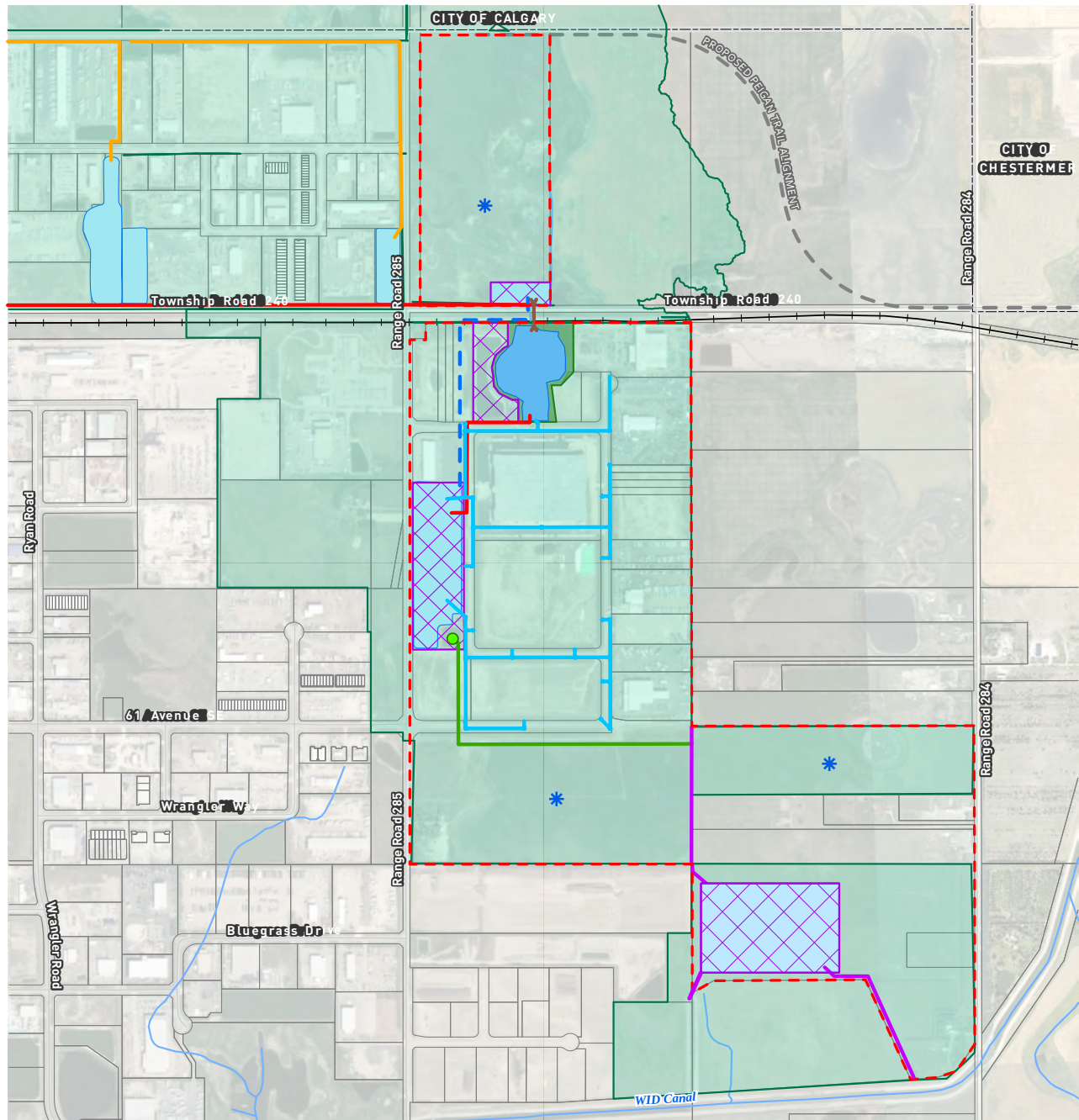
FIGURE 14 | ULTIMATE STORMWATER MANAGEMENT STRATEGY
